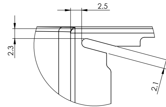
DETAIL M SCALE 2 : 1
